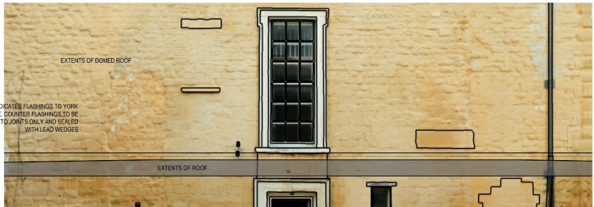
4 Elevation Detail 31 To York House - 1 to 50
