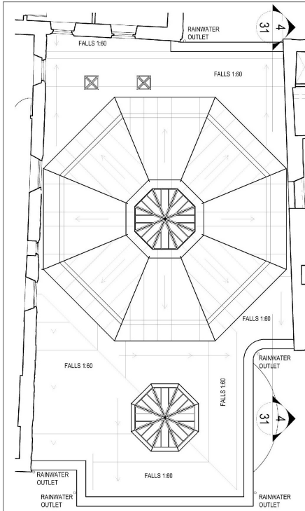
1 Roof Plan 31 1 to 100
