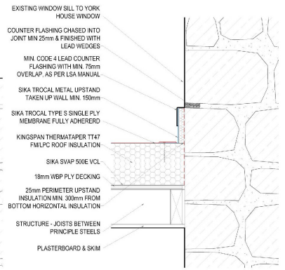
3 Section Detail 31 To York House Wall - 1 to 10
