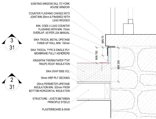
2 Section Detail 31 To York House Window - 1 to 10
